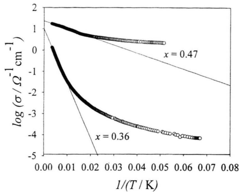
Fig. 6. Arrhenius plots for two non-superconducting samples of \text{SmBa}_2\text{Cu}_3\text{O}_{6+x} .
